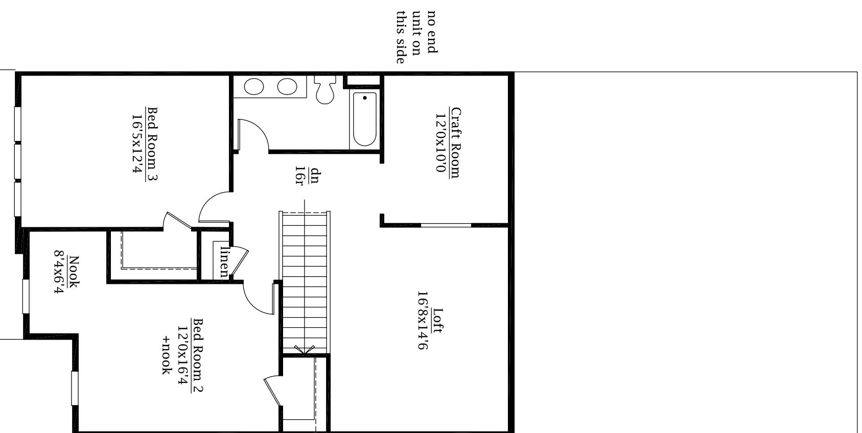
2nd Floor Plan with First Floor Owner's Suite Interior Unit/ Elev B shown - 1165 sq ft
