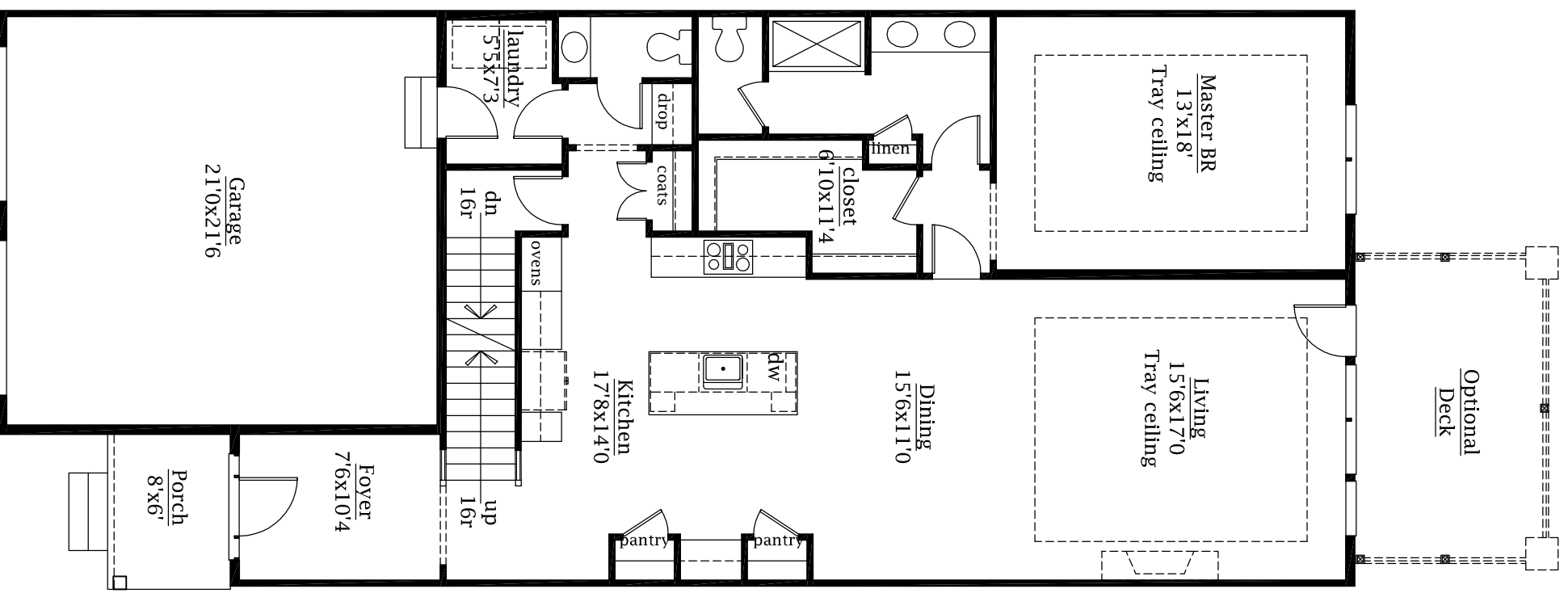
First Floor Plan with First Floor Owner's Suite Interior Unit 1475 sq. ft.
